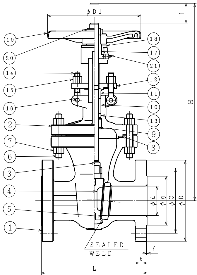
DIMENSIONS (mm)
