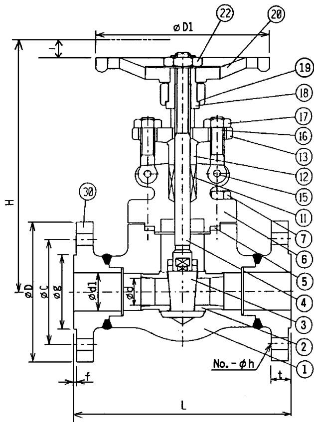
DIMENSIONS (mm)
